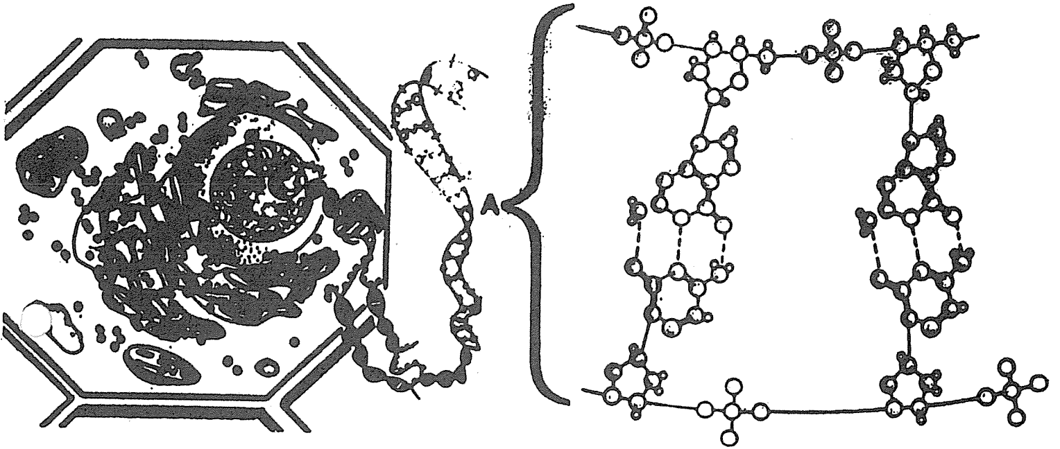
Figure 51. THE CHANCES OF CHANCE PRODUCING DNA
