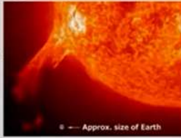
Right: An erupting solar prominence photographed by the Solar and Heliospheric Observatory (SOHO). [More ->]
