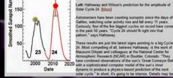
Left: Hathaway and Wilson's prediction for the amplitude of Solar Cycle 24. [More]
